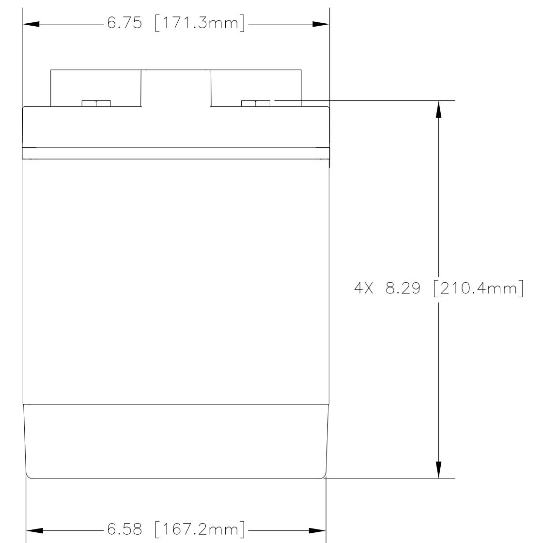
ENVELOPE DRAWING
