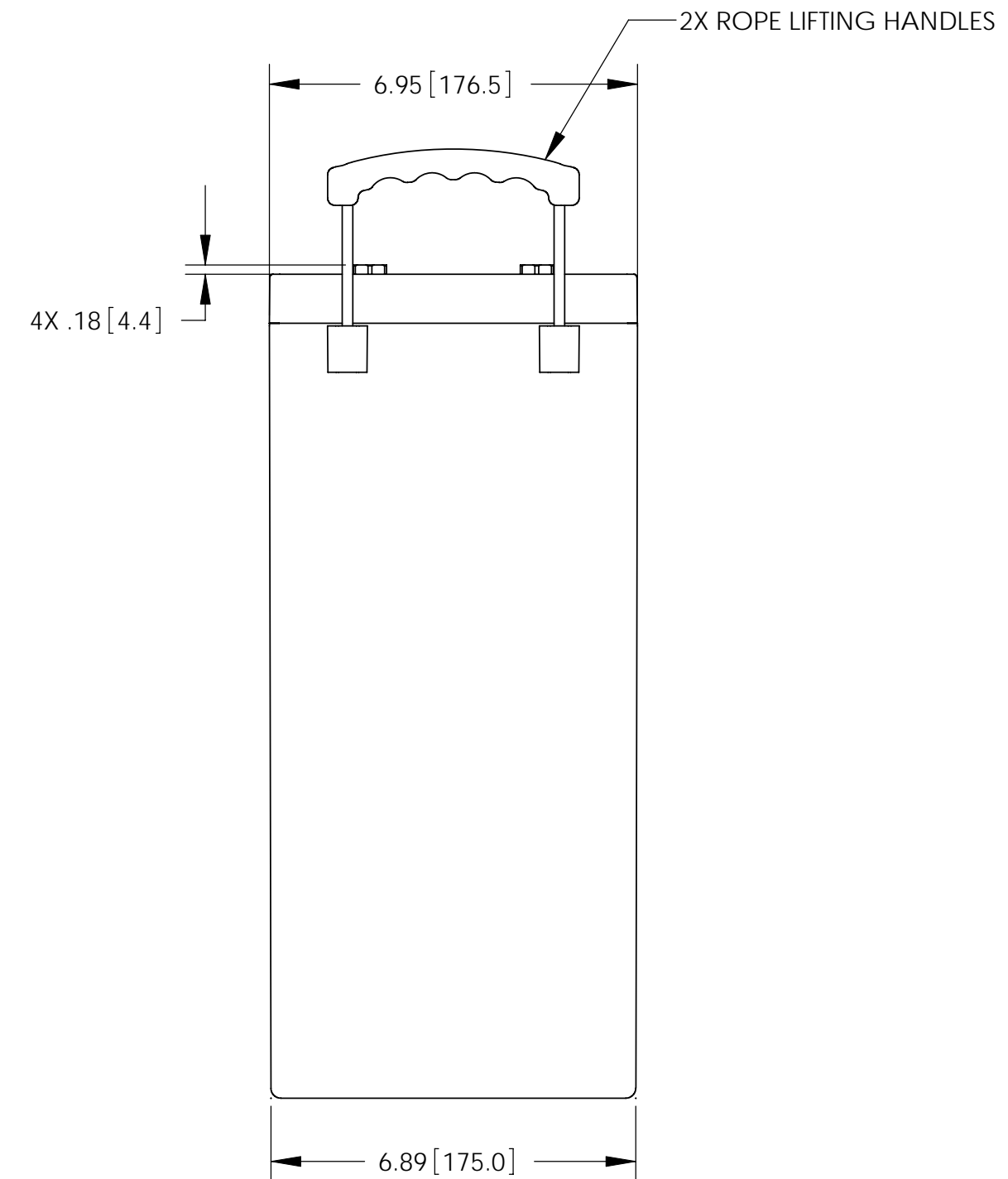
ENVELOPE DRAWING
